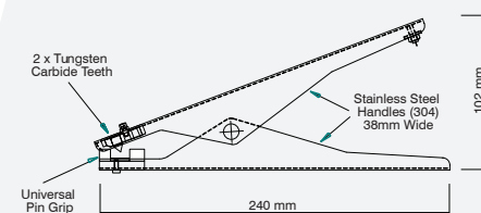
Static Grounding Clamp Dual core stainless steel grounding clamp fitted with one pair of tungsten carbide tips
