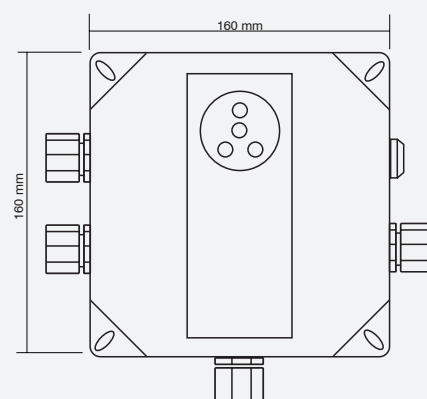
Earth-Rite II PLUS ground monitor-indicator station for Zone 0 and Zone 20 locations (or lower).
