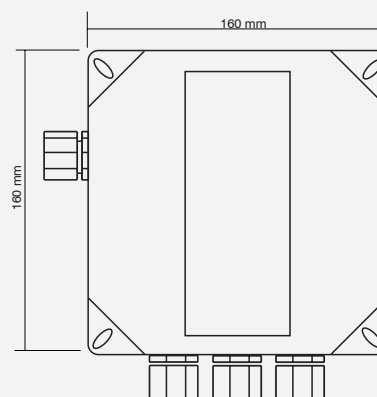
Earth-Rite II PLUS 240 V / 110 V AC power supply for Zone 2, 21, 22 or Non-Hazardous locations
