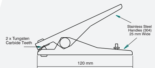
Static Grounding Clamp
